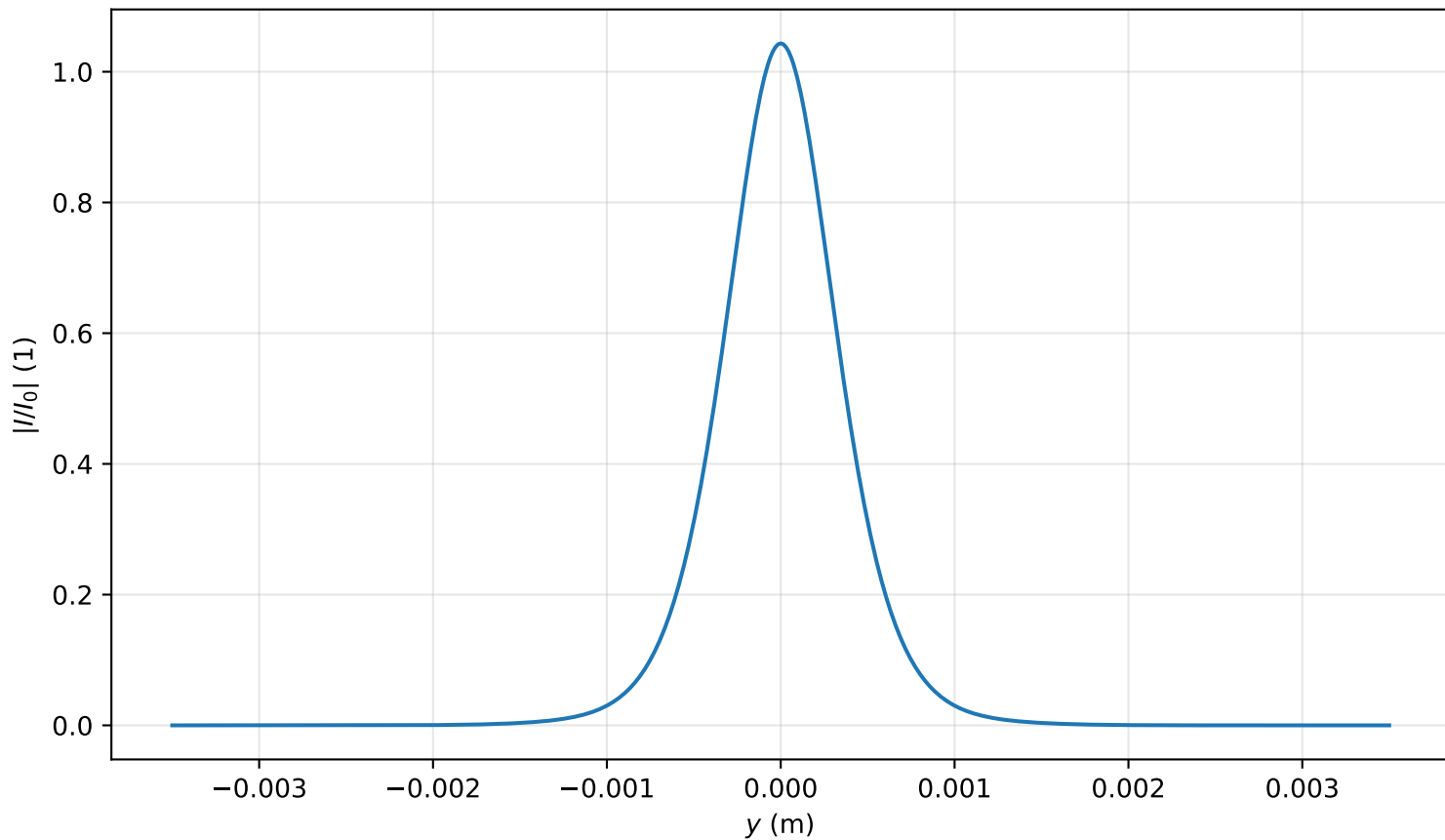
Intensity profile I(x=0, y, z=2.229)/I_0 , P_{in}=0.7P_{cr} , artificial time
